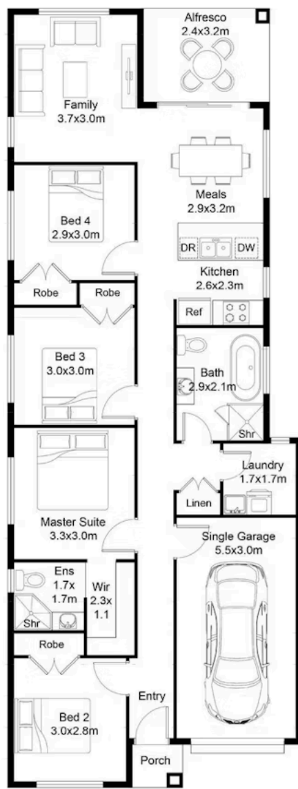
FLOOR PLAN
